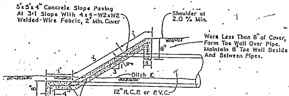
SLOPE PAVING DETAIL
