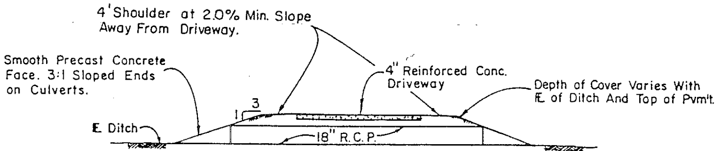
SECTION "A-A"
